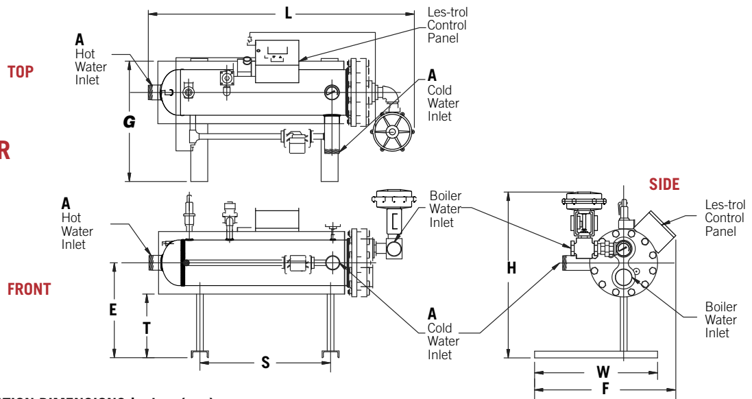
HORIZONTAL CONFIGURATION DIMENSIONS inches (mm)
