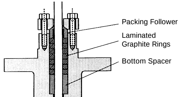
Figure 5 - Installation Sequence
