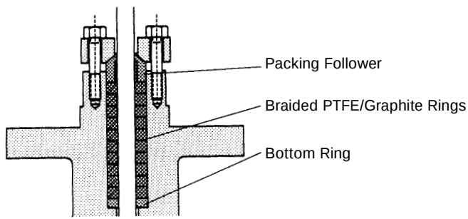
Figure 3 - Installation Sequence
