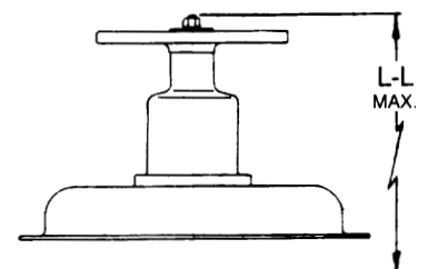
EXTERNAL VIEW OF HAND OPERATING DEVICE REVERSE ACTING
