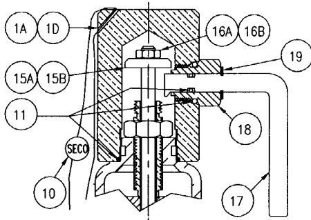
PACKED CAP OPTION
