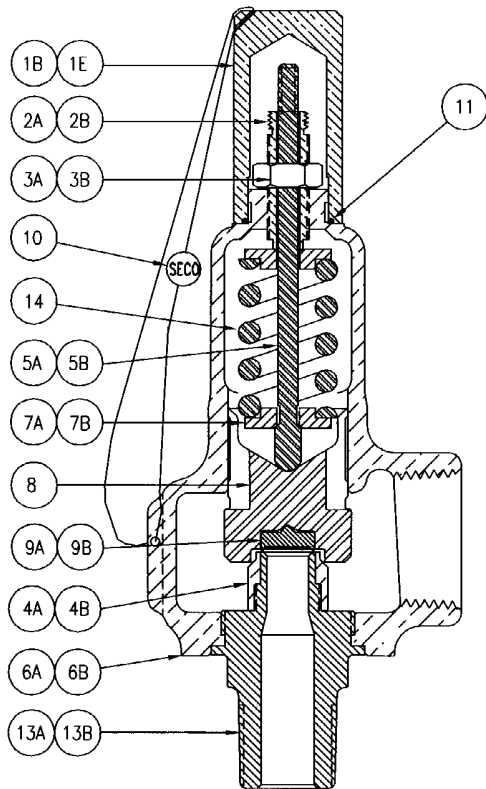
PLAIN CAP VALVE
