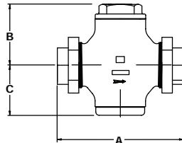
K1, K5 1/2" - 2"
