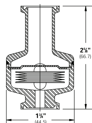
DS110 HYGIENIC CLAMP CONNECTION (1/2" & 3/4") Weight .4 lbs (0.18)
