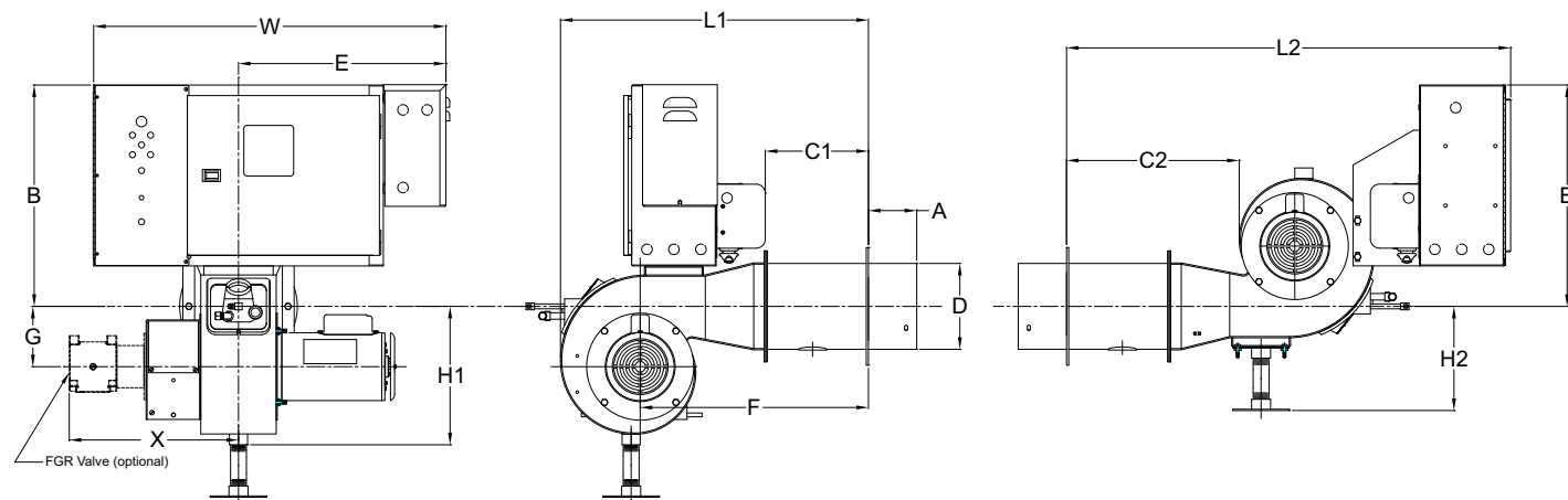
JB(X) STANDARD ARRANGEMENT
