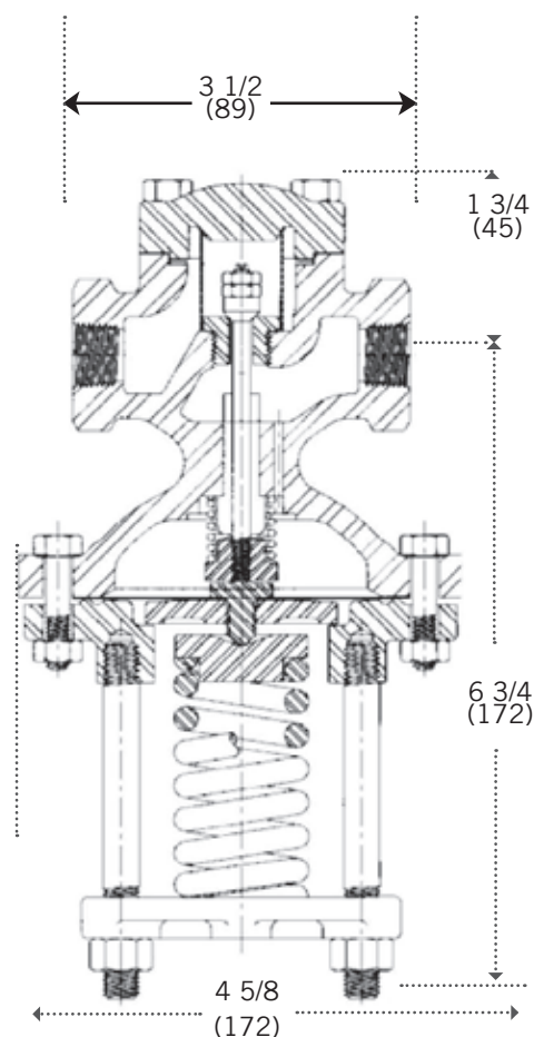
D VALVE 7.3 LBS. (3.3 KG)
