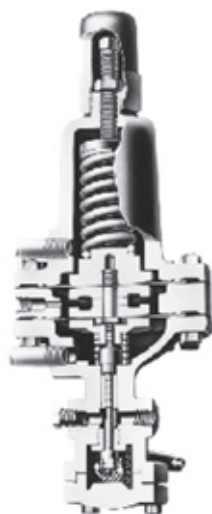
TYPE N33 PILOT
