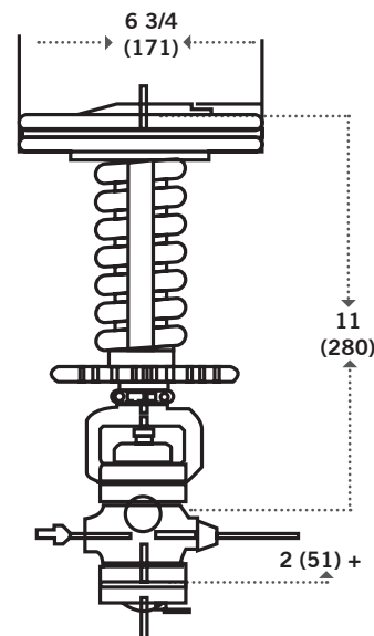
TYPE P15 PILOT 15 LBS. (6.8 KG)
