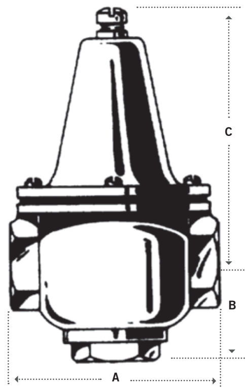
TYPE D36 WATER PRESSURE REDUCING VALVE
