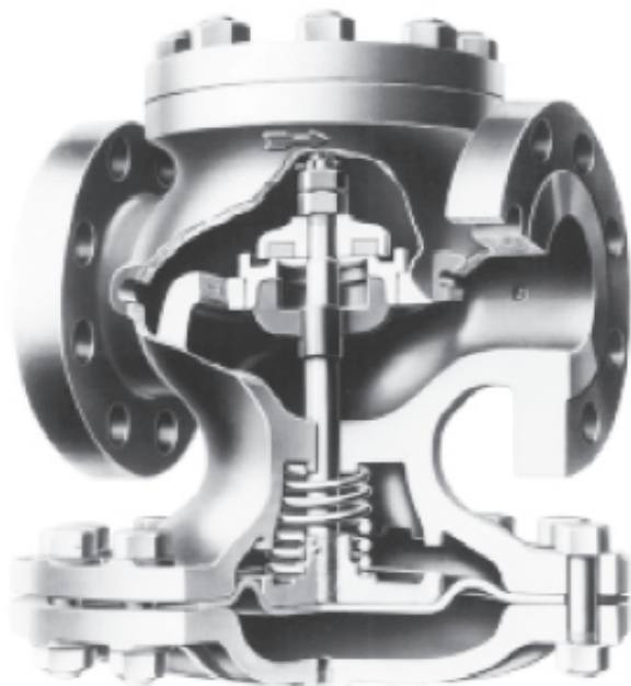
TYPE E6 MAIN VALVE
