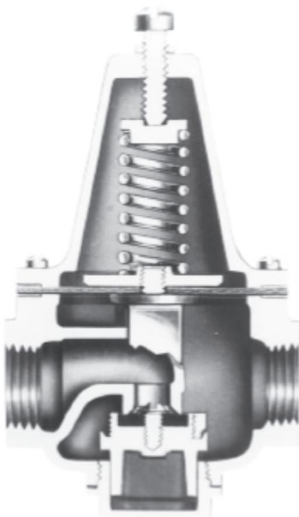
TYPE D36 WATER PRESSURE REDUCING VALVE
