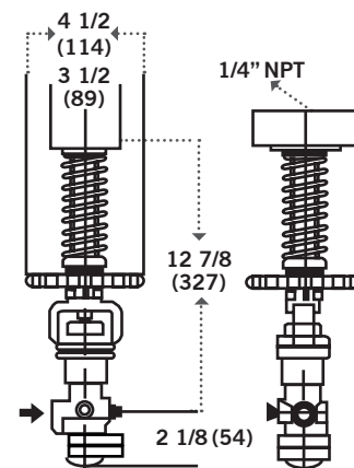
TYPE F32 PILOT 12 LBS (5.5 KG)
