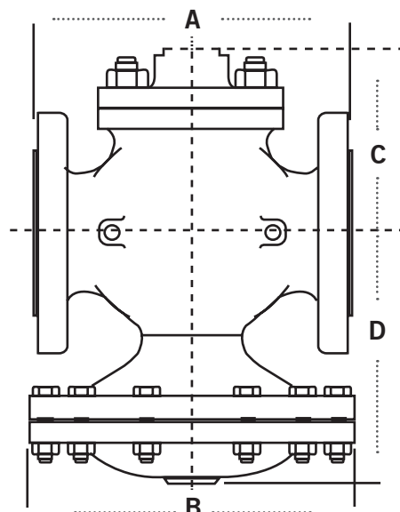
TYPE C34 MAIN VALVE
