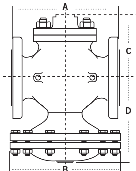
TYPE E6 MAIN VALVE
