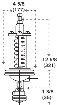
TYPE D2 10 LBS. (4.5 KG)
