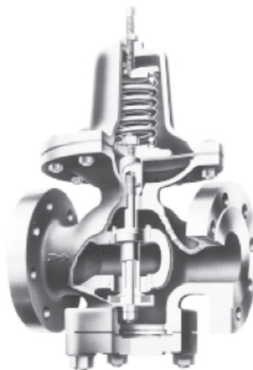
TYPE D34 WATER PRESSURE REDUCING VALVE
