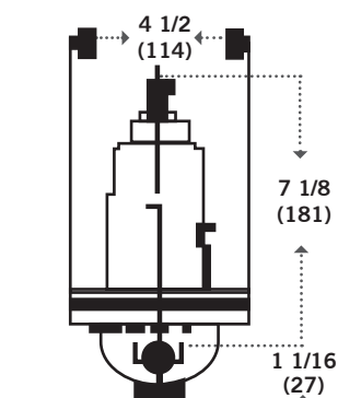
SPRING CHAMBER
