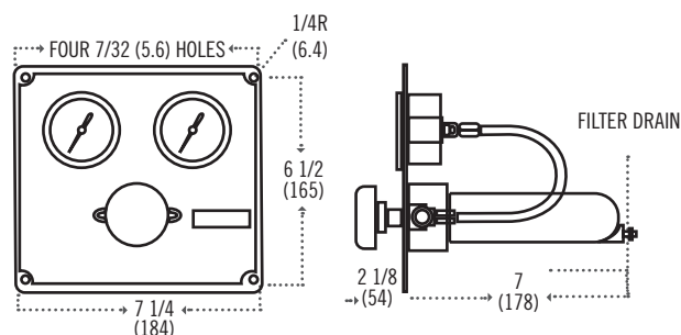
TYPE A PANEL cutout 5 1/4 (133) high by 6 (152) wide
