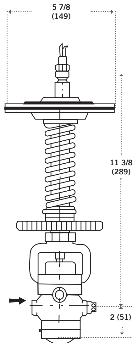
TYPE T14 TEMPERATURE PILOT 13 LBS. (6 KG)
