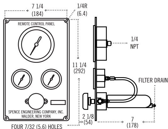
TYPE B PANEL cutout 10 1/4 (266) high by 6 (152) wide
