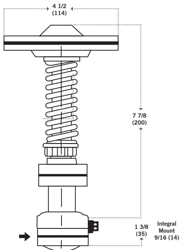
TYPE SP/P PRESSURE SAFETY PILOT 8 LBS. (3.6 KG)
