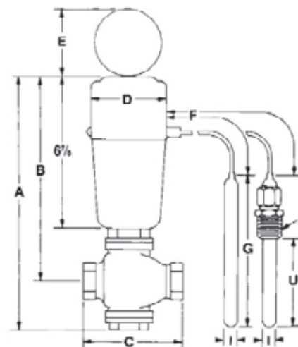
TYPE 2010-2040 DIRECT & REVERSE ACTING
