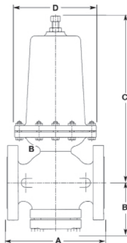
TYPE D34 WATER PRESSURE REDUCING VALVE
