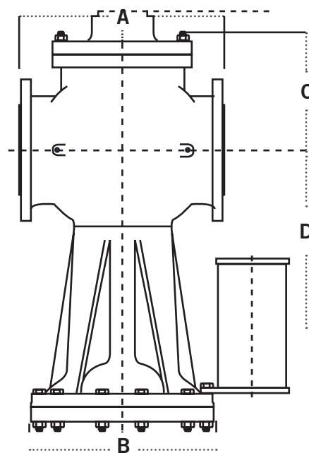
TYPE E5 MAIN VALVE
