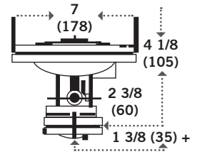
TYPE A83 11 LBS (5 KG)
