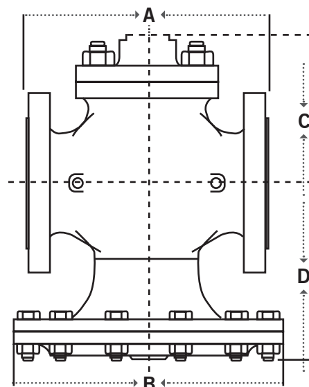
TYPE E MAIN VALVE
