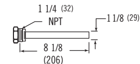
727 WELL - Used with 704 Bulb
