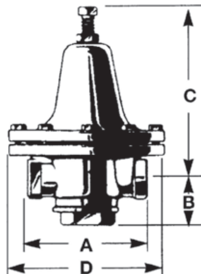
TYPE D50 DIRECT ACTING PRESSURE REDUCING VALVE
