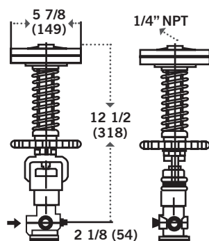
TYPE F14 PILOT 14 LBS (6.4 KG)
