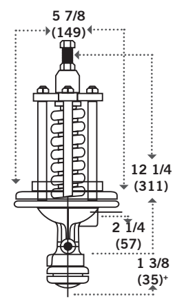
TYPE D120 16 LBS. (7.3 KG)
