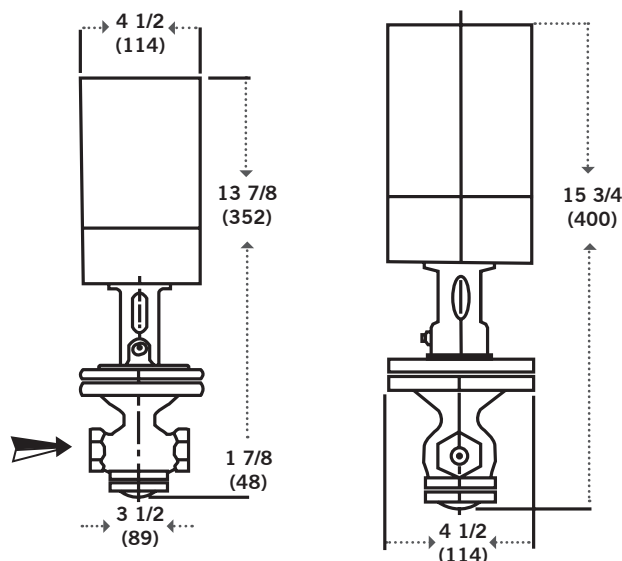
TYPE D210 ELECTRONIC ACTUATOR PILOT
