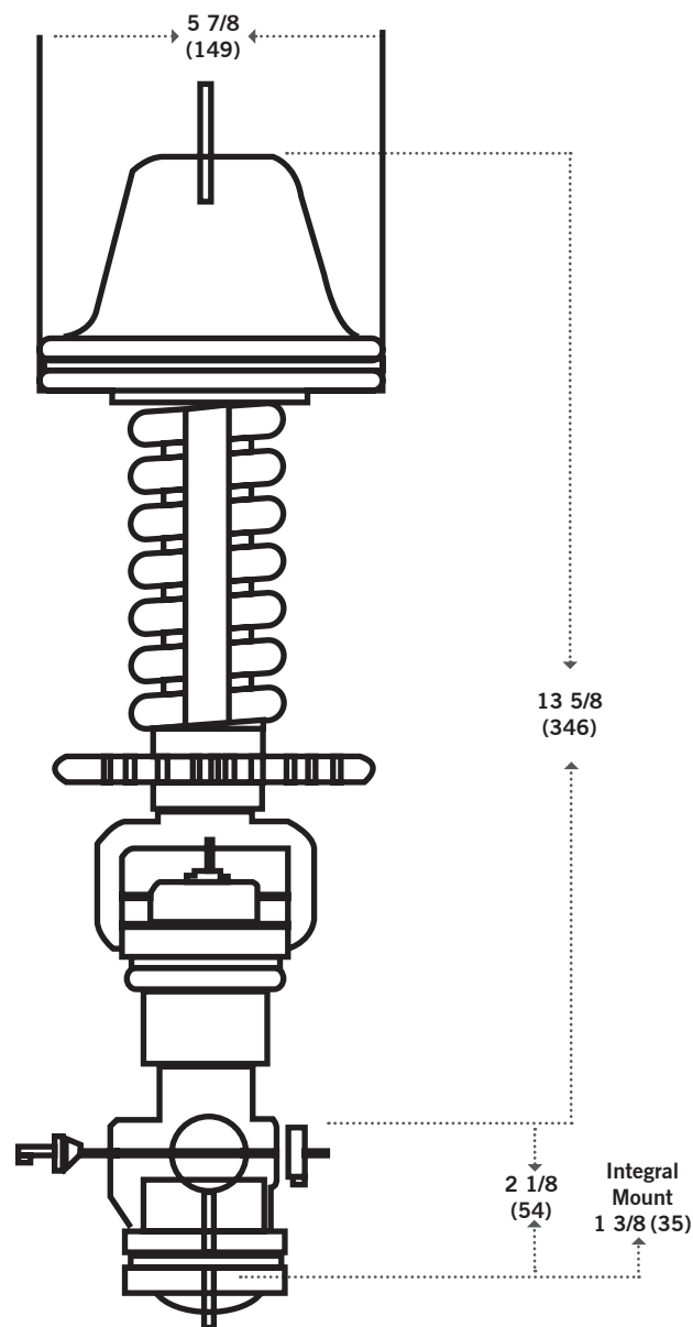
TYPE F46 PILOT 15 LBS (6.8 KG)
