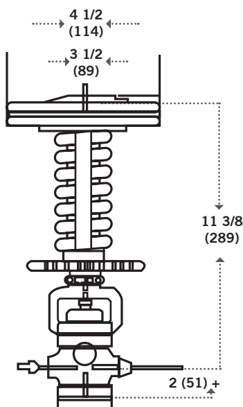
TYPE P32 PILOT 10 LBS. (4.5 KG)
