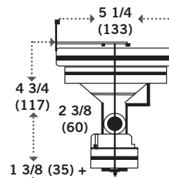
TYPE A43 11 LBS (5 KG)
