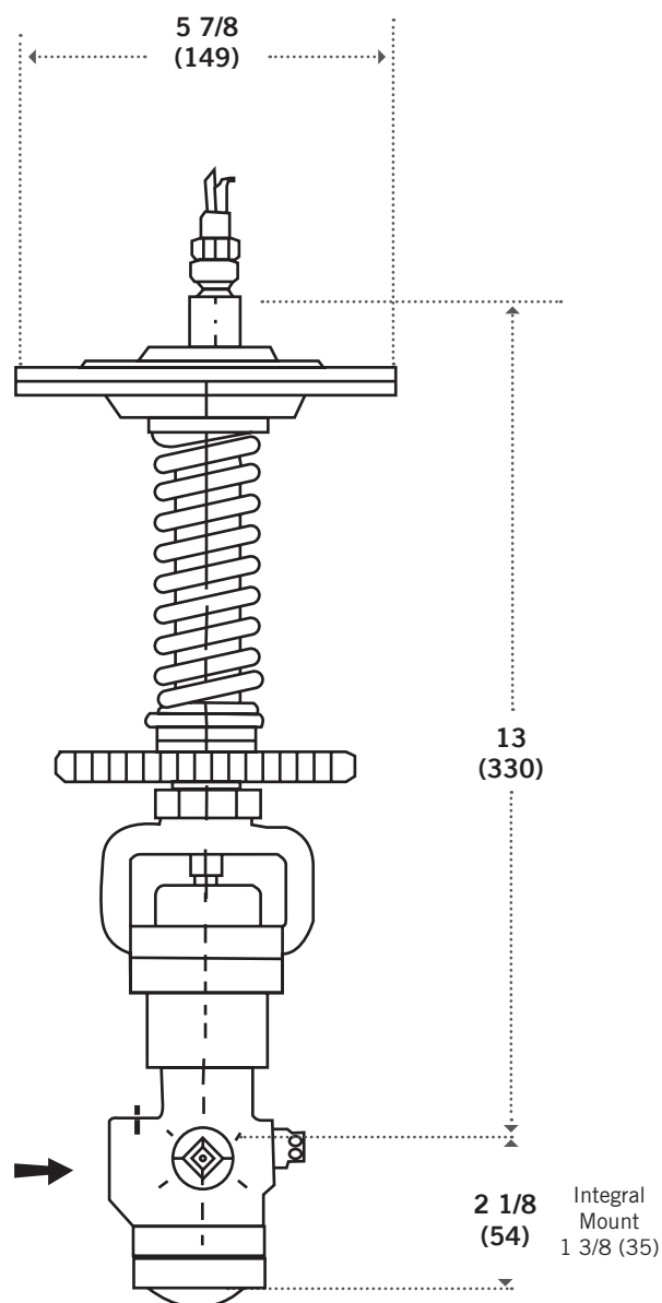
TYPE T52 PILOT 14 LBS. (6.4 KG)
