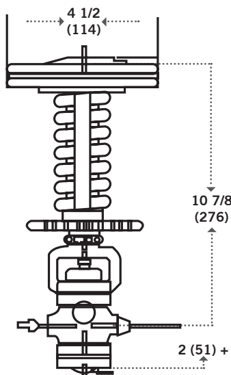
TYPE P13 PILOT 11 LBS. (5 KG)
