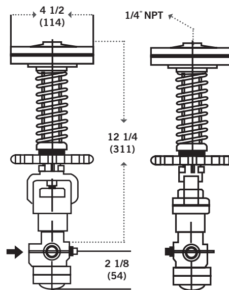
TYPE F13 PILOT 12 LBS (5.5 KG)
