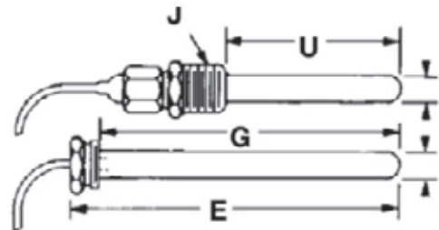
GAS SERVICE BULB & WELL DIMENSIONS INCHES (MM)
