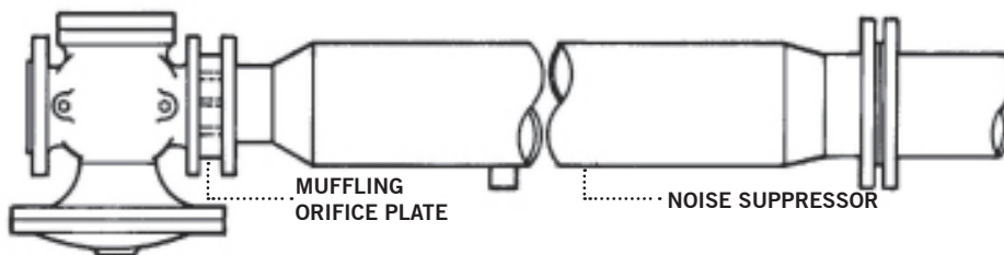
FIGURE 5C: SINGLE STAGE INSTALLATION WITH MUFFLING ORIFICE AND NOISE SUPPRESSOR
