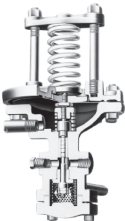
TYPE D PRESSURE PILOT
