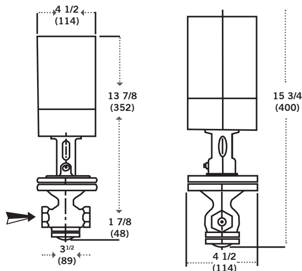
TYPE D208 ELECTRONIC ACTUATOR PILOT
