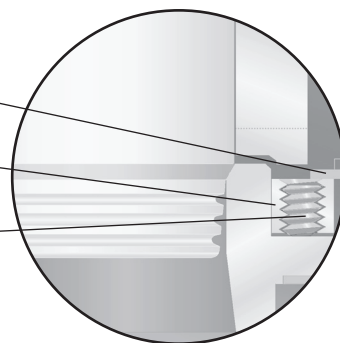
Load Ring Detail (Cage Throttling 4" Valve Size Only)
