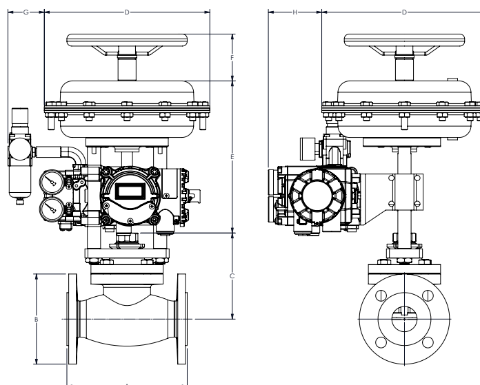
Diaphragm Actuator Pillar Yoke
