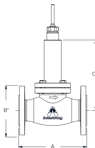
Bellow Seal - Cryogenic** - LeakOff** Bonnet
