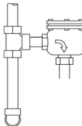
Figure 5. Dirt pocket made from pipe fittings when a strainer is not available. Clean dirt pockets and strainers frequently.
