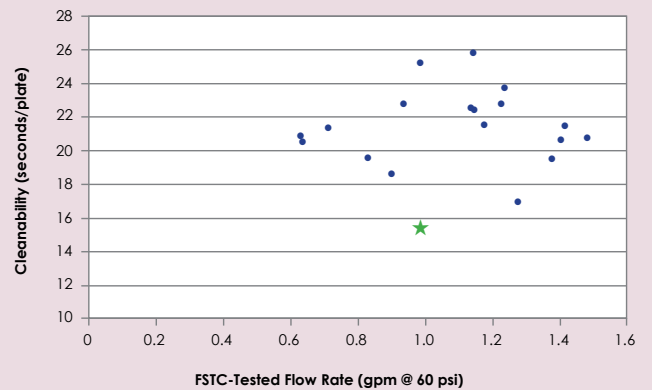
FSTC-Tested Flow Rate vs. Cleanability
